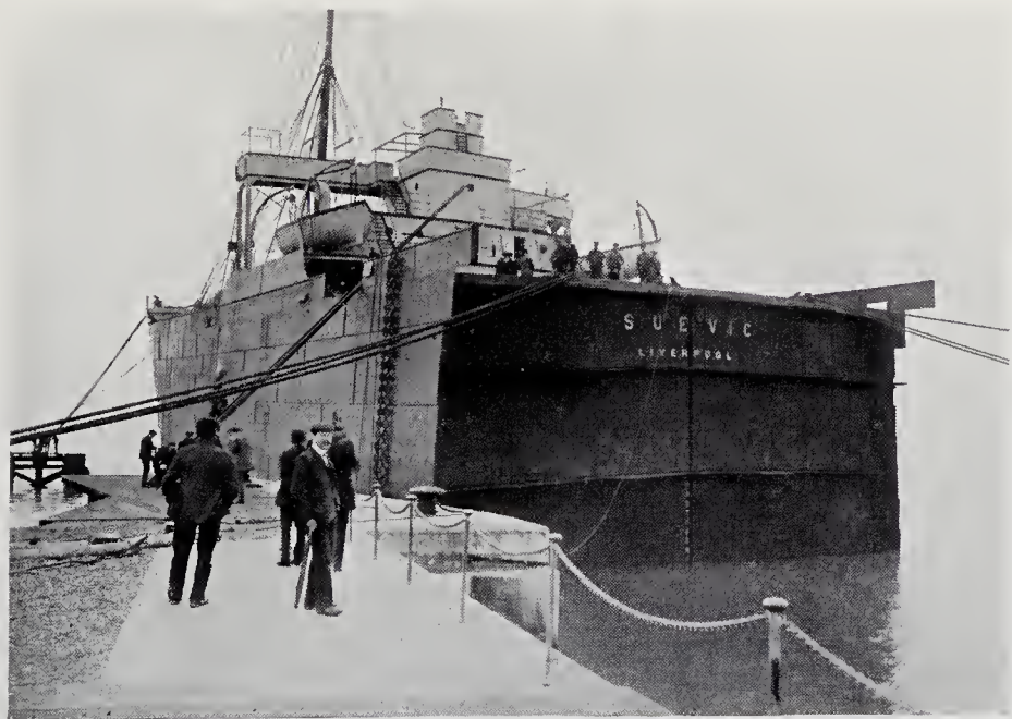
THE NEW BOW OF THE "SUEVIC" AT ENTRANCE TO DOCK. From Photographs by Reginald Silk, Portsmouth.
