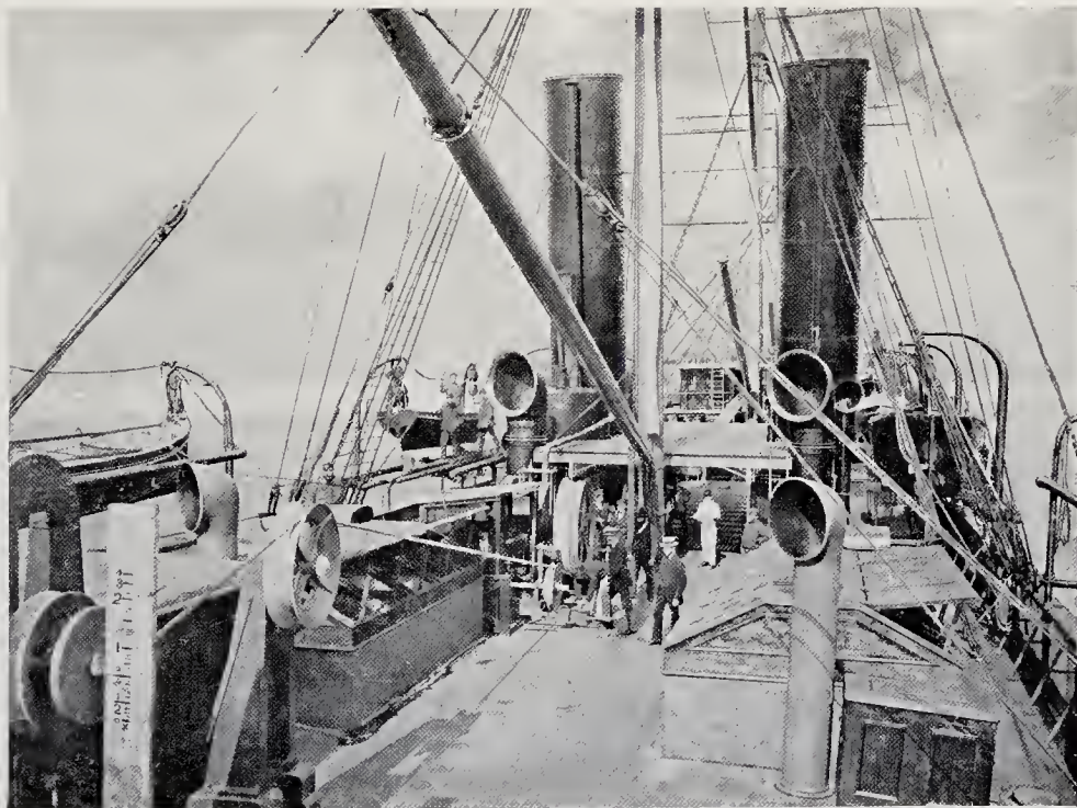
DECK VIEW OF THE TELEGRAPH SHIP "FARADAY." From a Photograph. By permission of Messrs. Siemens & Co.
