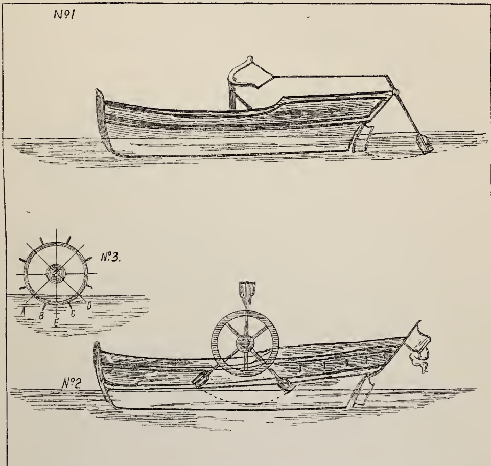
FULTON'S FIRST PLANS FOR STEAM NAVIGATION
