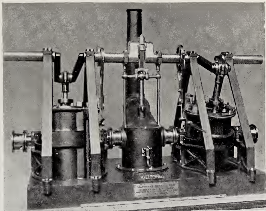
MAUDSLAY'S OSCILLATING ENGINE. From the Original in the Victoria and Albert Museum.
