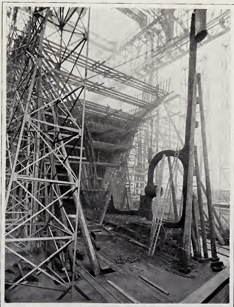
STERN FRAME OF THE "TITANIC," FEB. 9, 1910.
