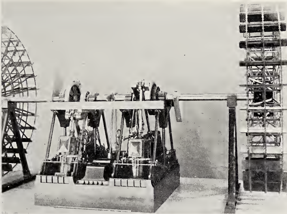
PADDLE ENGINES OF THE "GREAT EASTERN."
