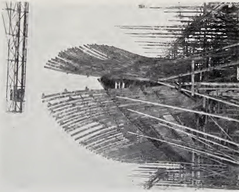
BOWS OF THE "BERLIN" IN COURSE OF CONSTRUCTION.
