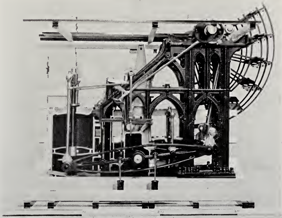
SIDE-LEVER ENGINE. From the Model in the Victoria and Albert Museum.
