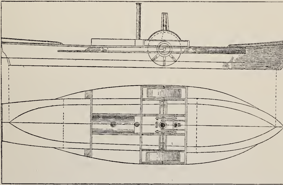
FULTON'S PLANS OF A LATER STEAMBOAT THAN THE CLERMONT-NORTH RIVER , SHOWING APPLICATION OF THE SQUARE SIDE-CONNECTING-ROD ENGINE.
