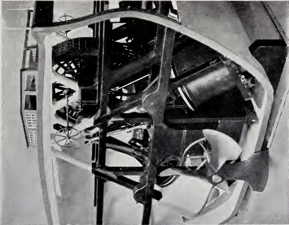
ENGINES OF THE "GREAT BRITAIN."
