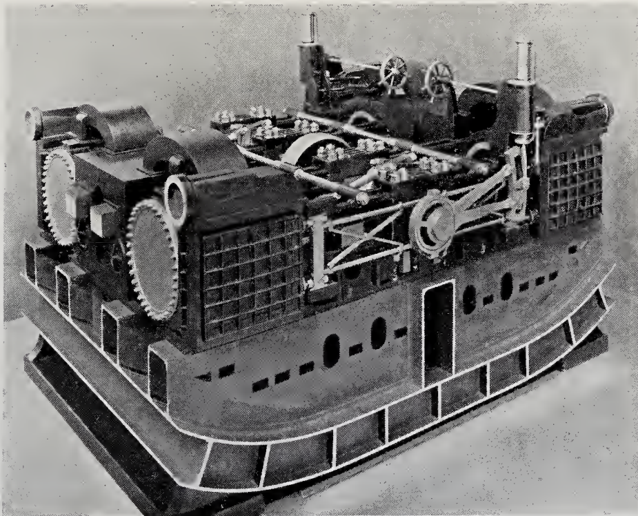
SCREW ENGINES OF THE "GREAT EASTERN."
