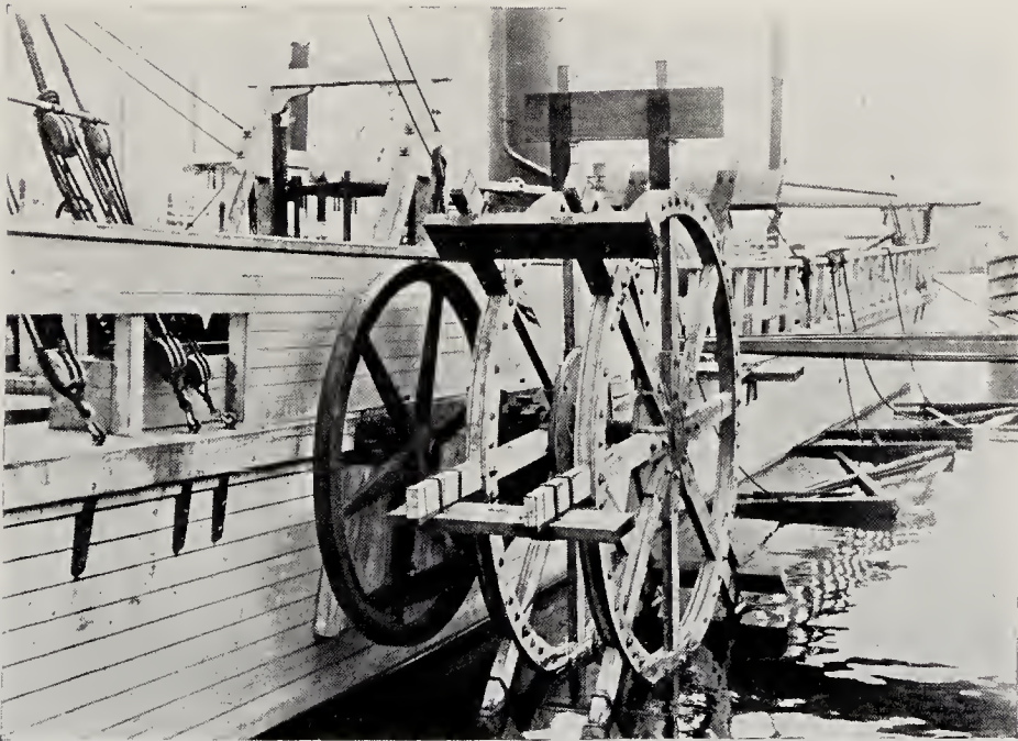
PADDLE-WHEEL OF THE RECONSTRUCTED "CLERMONT."
