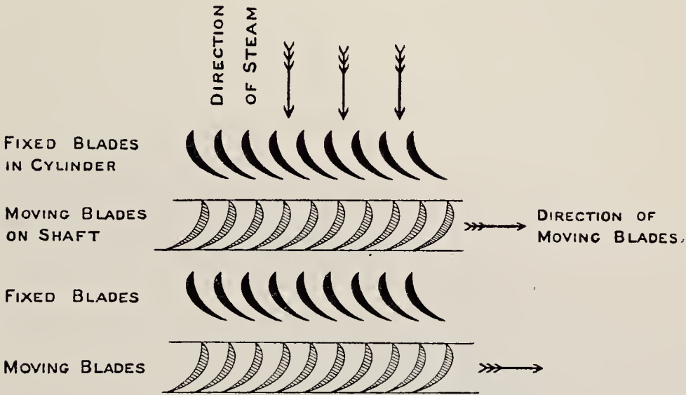
THE BLADES OF A PARSONS TURBINE.
