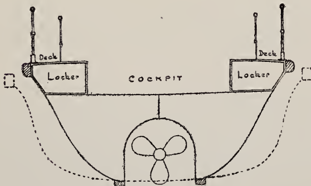
SECTION THROUGH TUNNEL.
