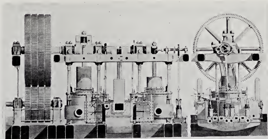
ENGINES OF THE "CANDIA." From the Drawing in the Victoria and Albert Museum.
