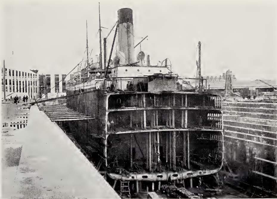
THE STERN PART OF THE "SUEVIC" AWAITING THE NEW BOW AT SOUTHAMPTON.
