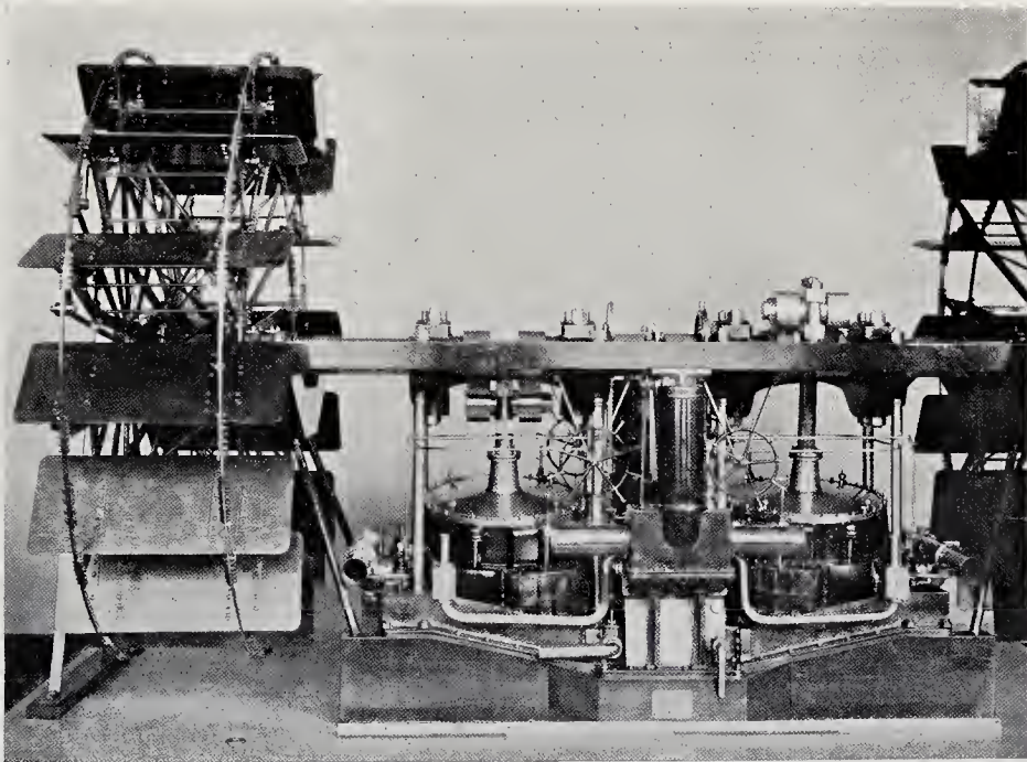
ENGINES OF THE "LEINSTER" (1860).
