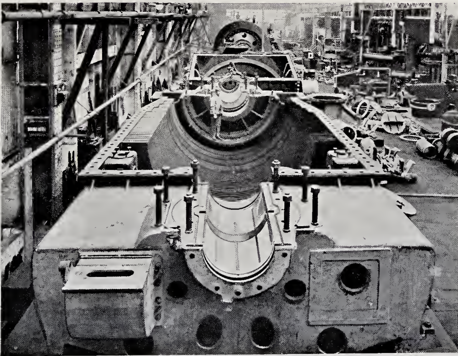
LOWER HALF OF THE FIXED PORTION OF ONE OF THE "CARMANIA'S" TURBINES.
