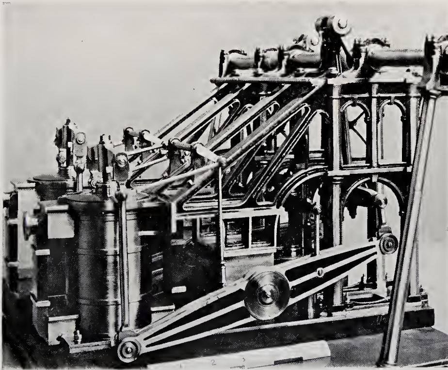
SIDE-LEVER ENGINES OF THE "RUBY" (1836).
